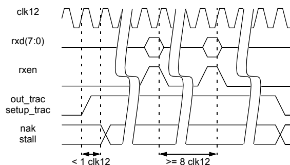
Figure 2: Endpoint Bus: Receive Timing.
