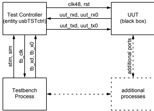
Figure 10: Simulation: Testbench Setup.
