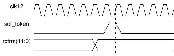
Figure 4: Endpoint Bus: SOF Token.
