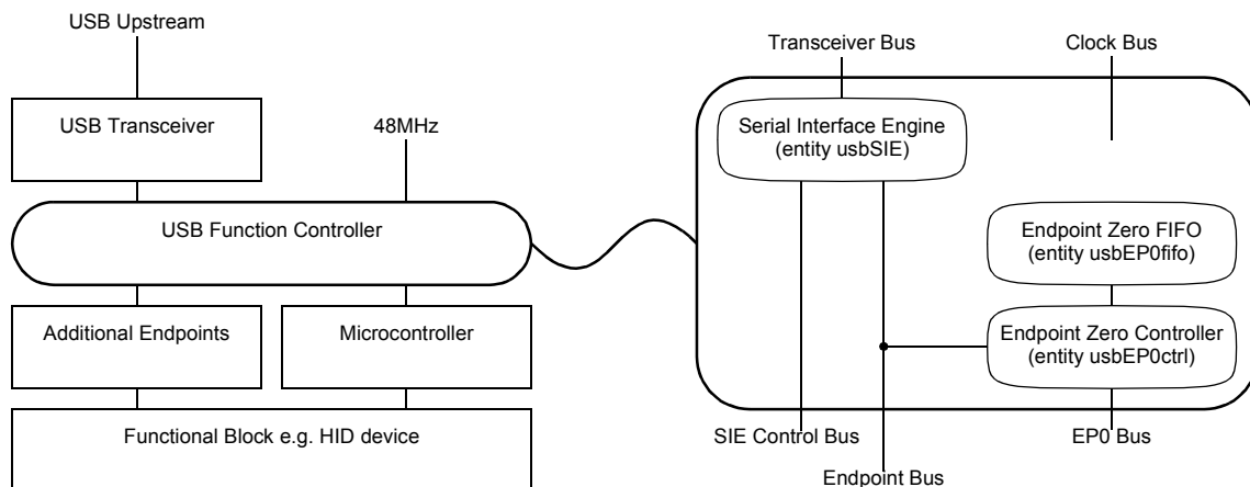
Figure 1: System architecture.
