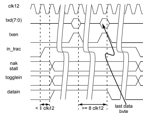
Figure 3: Endpoint Bus: Transmit Timing.
